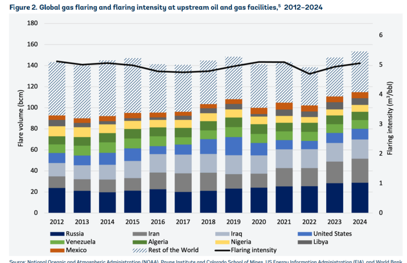
Figure 2. Global gas flaring and flaring intensity at upstream oil and gas facilities, 2012-2024. Source: National Oceanic and Atmospheric Administration (NOAA), Paine Institute and Colorado School of Mines, US Energy Information Administration (EIA), and World Bank.
