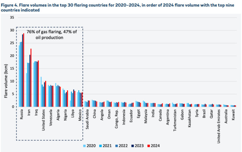
Figure 4. Flare volumes in the top 30 flaring countries for 2020-2024, in order of 2024 flare volume with the top nine countries indicated. Source: NOAA, Paine Institute and Colorado School of Mines, and World Bank.
